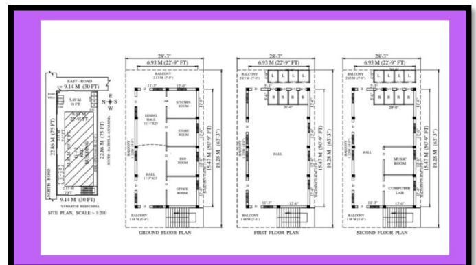
Purposed new building engineer plan
