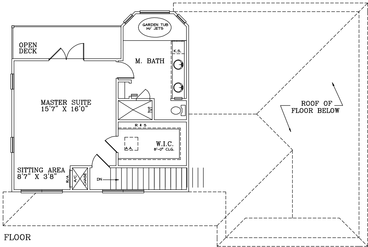
FIRST FLOOR
